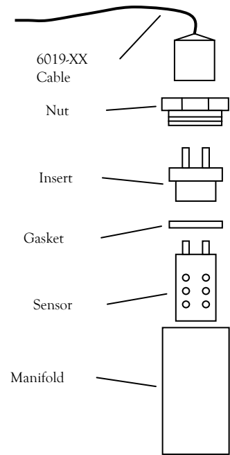
Remote Sensor Installation
