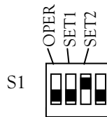
S1 Settings for Relay #2 setpoint view and adjustment
